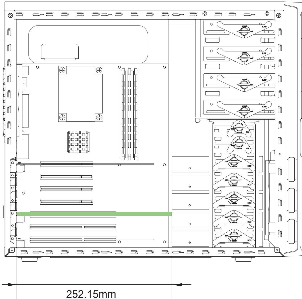
Maximum width for VGA Card
