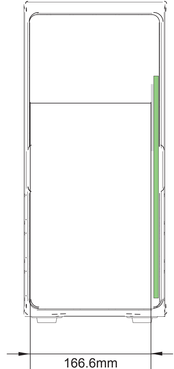
Maximum height for CPU Cooler
