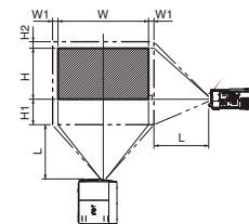
Front projection
