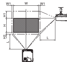
Front projection, ceiling mounting
